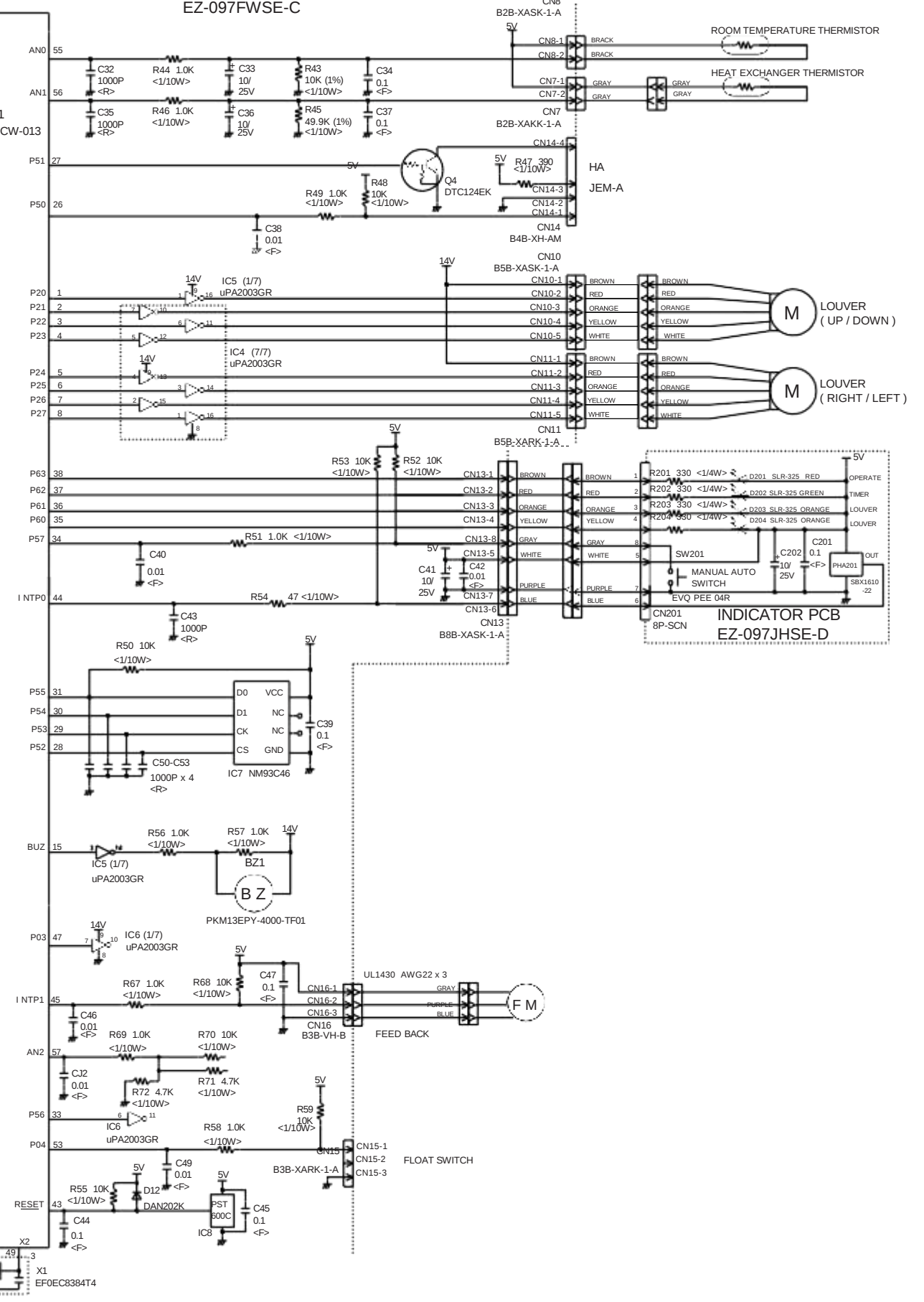
CONTROLLER PCB ASSEMBLY ( MAIN PCB ) EZ-097FWSE-C
